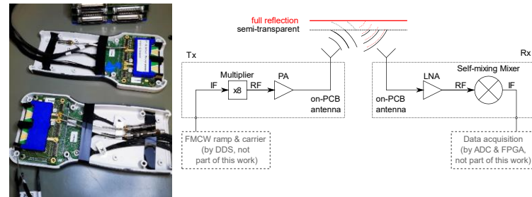
Self-mixing radar demonstrator frontend (E-band) and scheme with independent Tx and Rx
