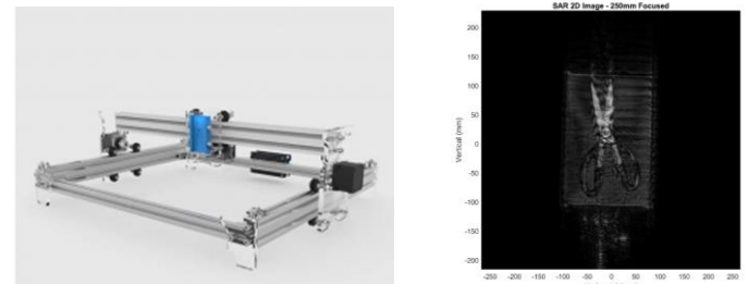
Exemplary scanner hardware and radar image
